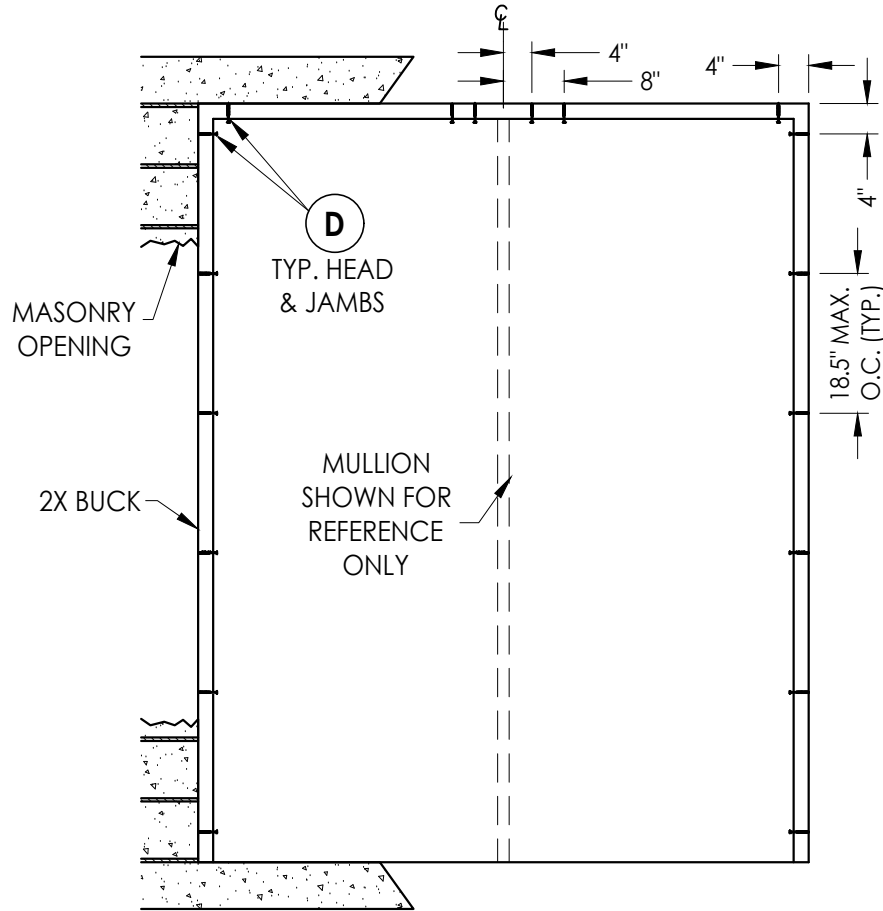
BUCK ANCHORING
