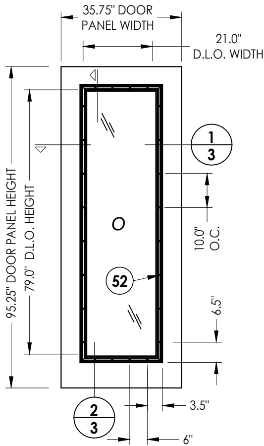
50 SIDELITE PANEL
