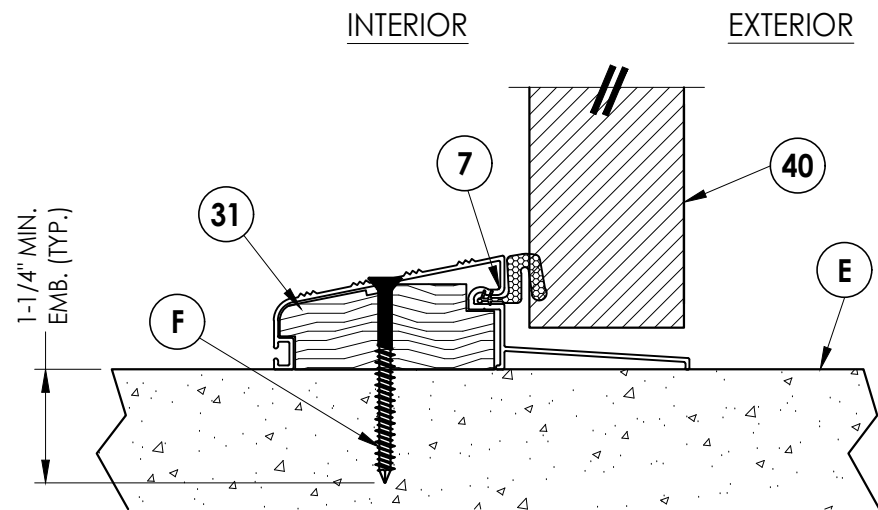
2 6 VERTICAL CROSS SECTION Shown w/1X sub-buck
