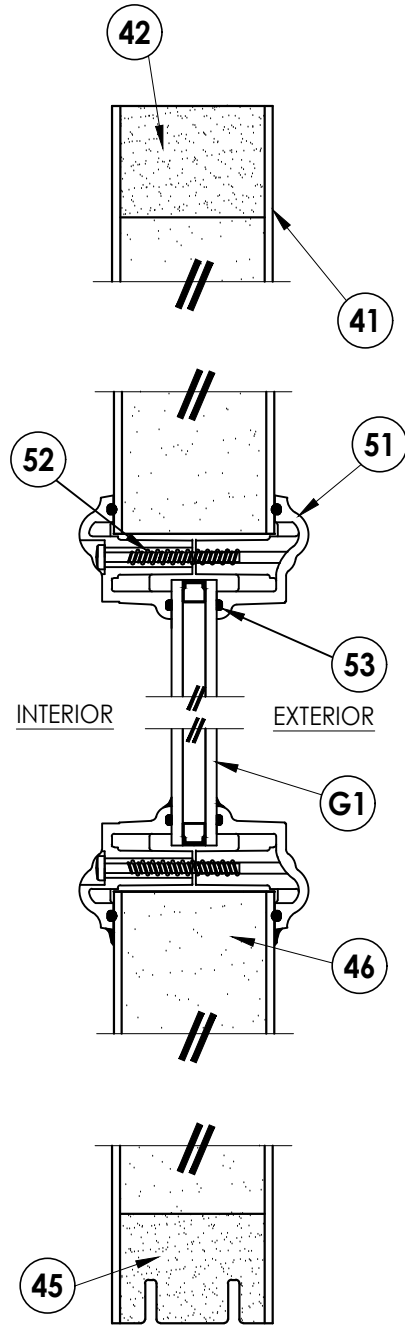
2/3 VERTICAL CROSS SECTION
